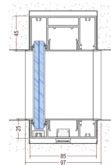
metrica® fA Asymmetrical glazed partition. Concealed profile.
