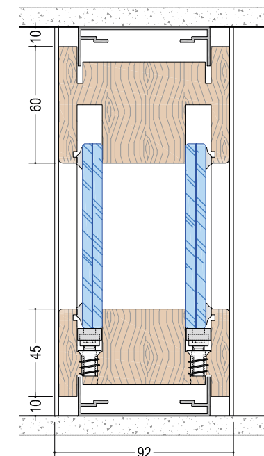
ritmica® wood d2 Double glazed partition.
