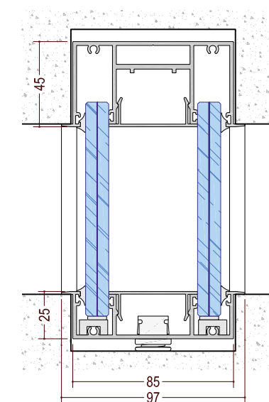
metrica® f2 Double glazed partition. Concealed profile.
