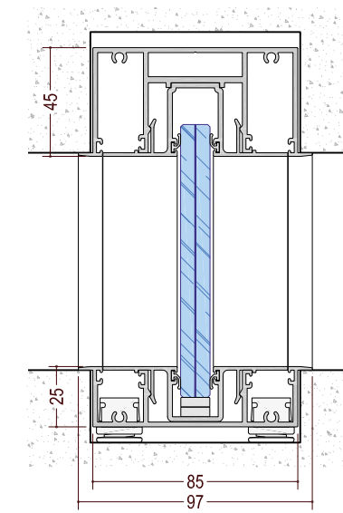
metrica® f1 Central glass partition. Concealed profile.
