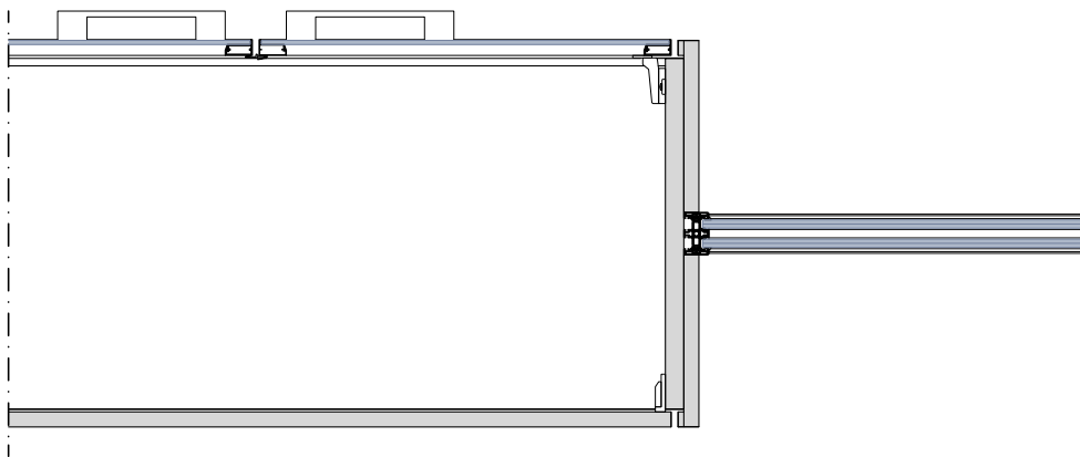
Central junction with unica d, recessed
