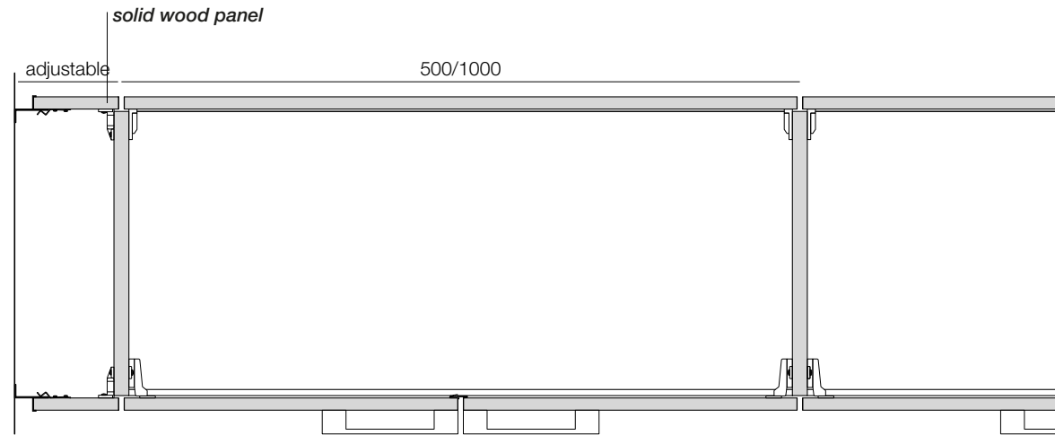
Wall-end upright with filler panel
