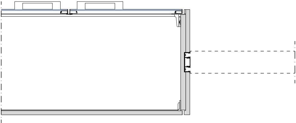
Central junction with Metrica Without Uprights, recessed
