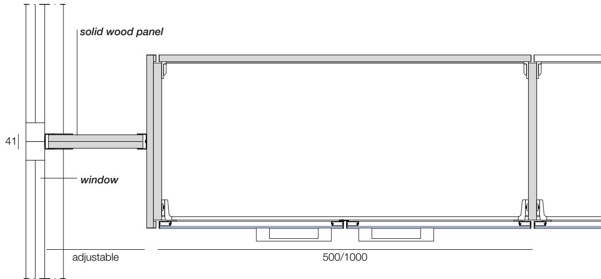
Wall-end upright
