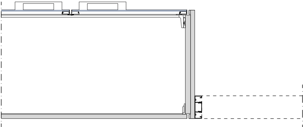
Straight junction with Metrica Without Uprights
