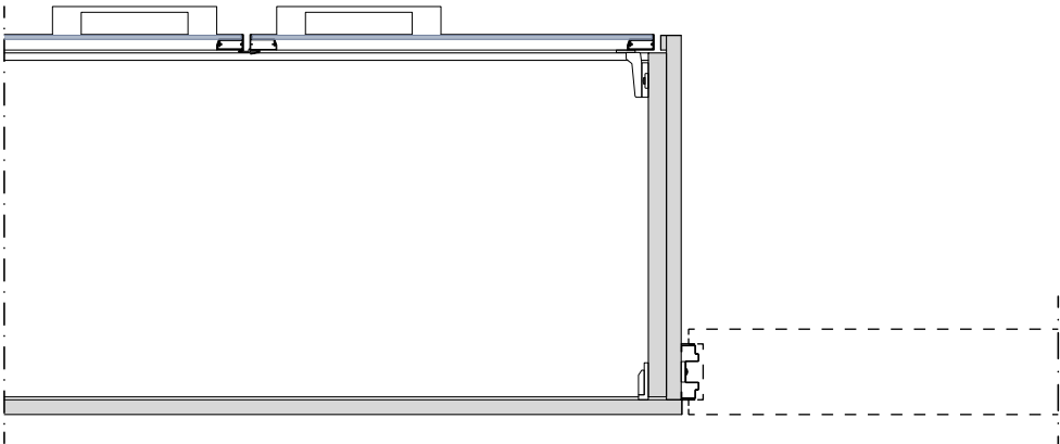
Straight junction with Metrica Structural
