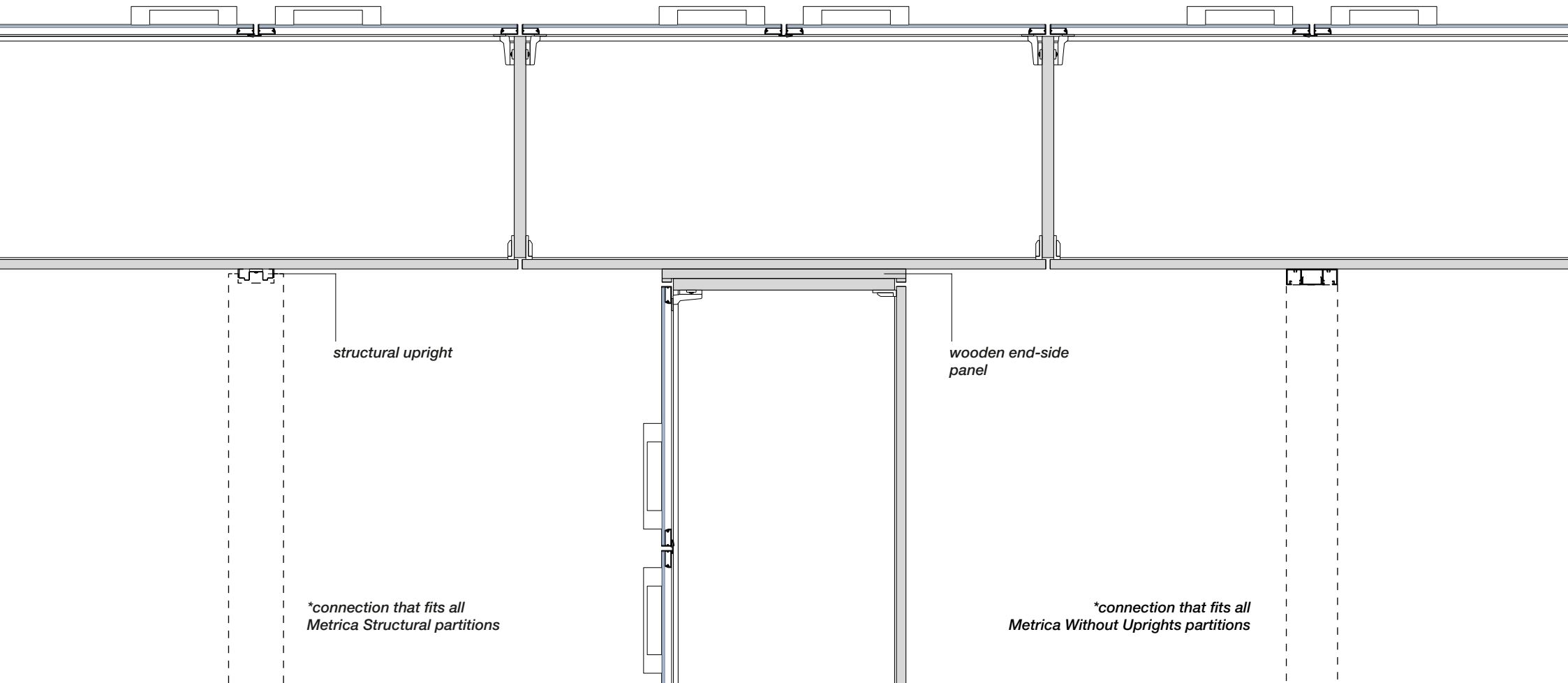
Three-way junction with Metrica Structural
