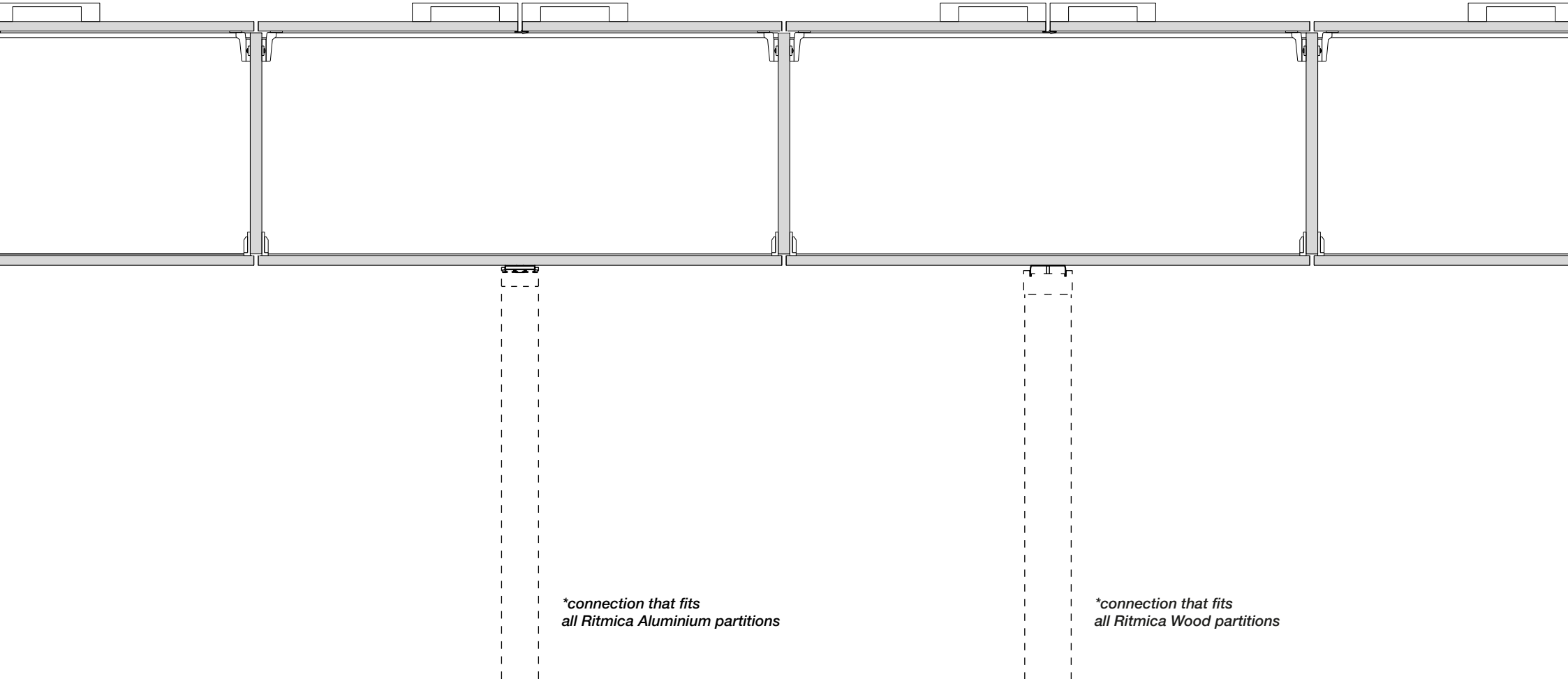
Three-way junction with Ritmica Aluminium
