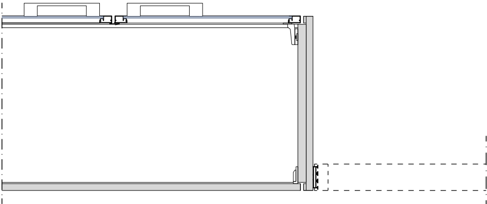
Straight junction with Ritmica Aluminium
