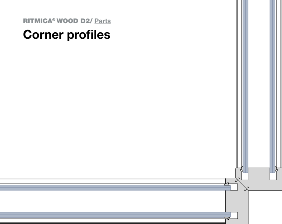
Wooden 90° corner profile double glass
