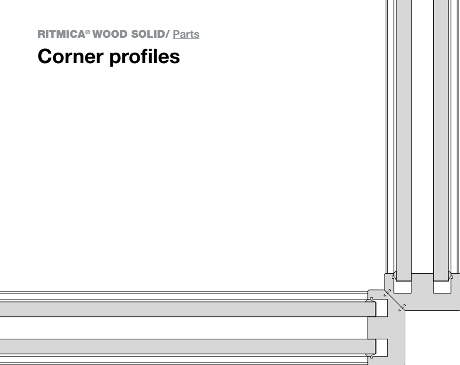
Wooden 90° corner profile double solid panel
