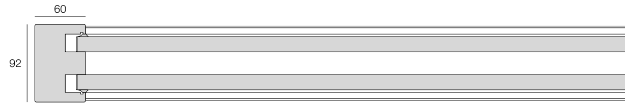
End profile
