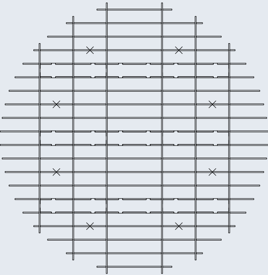
02 2720x2740 mm
